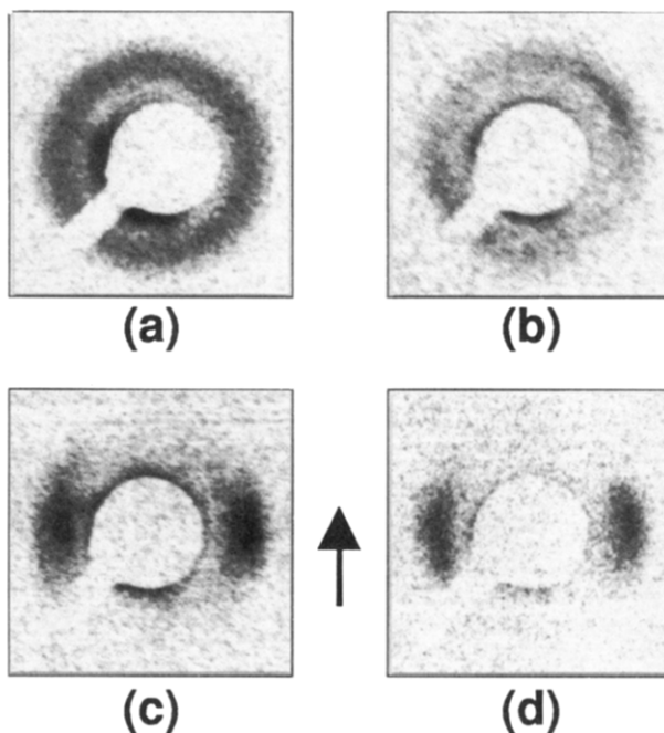
Figure 3. SAXS patterns from block copolymer samples after cooling from (a) 265 °C and (b) 281 °C in the absence of an electric field. (c) and (d) are of the same samples, respectively, but after a second identical thermal cycle where a 17.7 kV/cm electric field was applied during cooling. The arrow indicates the direction of the applied field during poling in (c) and (d).
